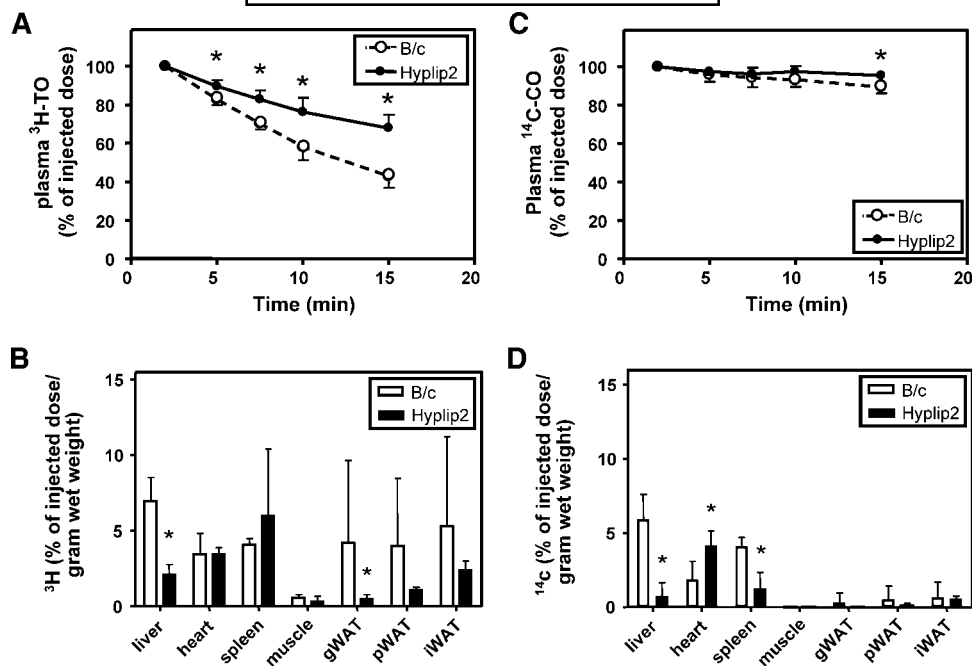
Fig. 5. Effect of Hyplip2 locus on plasma clearance (A, C) and organ distribution (B, D) of VLDL-like emulsion particles in vivo. [ 3 H]TG and cholesteryl [ 14 C]oleate ([ 14 C]CO) double-labeled emulsion particles (1 mg of TG) were injected via the vena cava inferior into anesthetized B/c and Hyplip2 mice. Blood samples were taken at the indicated time points, and 3 H activity (A) and 14 C activity (C) were determined in plasma. After 15 min, mice were euthanized, and organs were isolated, dissolved in Soluene, and counted for 3 H activity (B) and 14 C activity (D). Values are corrected for entrapped plasma and are means ± SD (n = 4 per group). * P < 0.05. gWAT, iWAT, and pWAT, gonadal, intestinal, and perirenal white adipose tissue.
