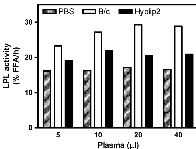
Fig. 9. Effect of Hyplip2 locus on bovine LPL activity. Plasma was obtained from eight Hyplip2 and eight B/c mice after 4 h of fasting and pooled per group. Endogenous LPL was heat-inactivated, and 5, 10, 20, and 40 \mu l of plasma was added to a mixture of glycerol [ 3 H]TO-labeled VLDL-like emulsion particles, FA-free BSA, and bovine LPL. TG hydrolase activity was calculated as the percentage of [ 3 H]oleate produced per hour.
